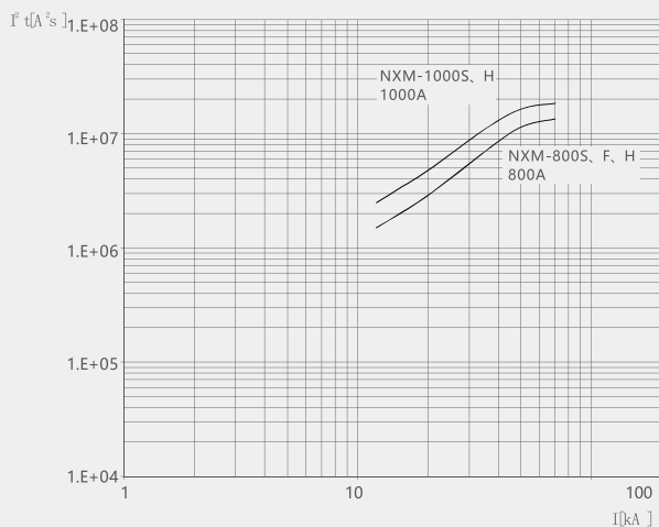
NXM-800/1000 let-through energy curve
