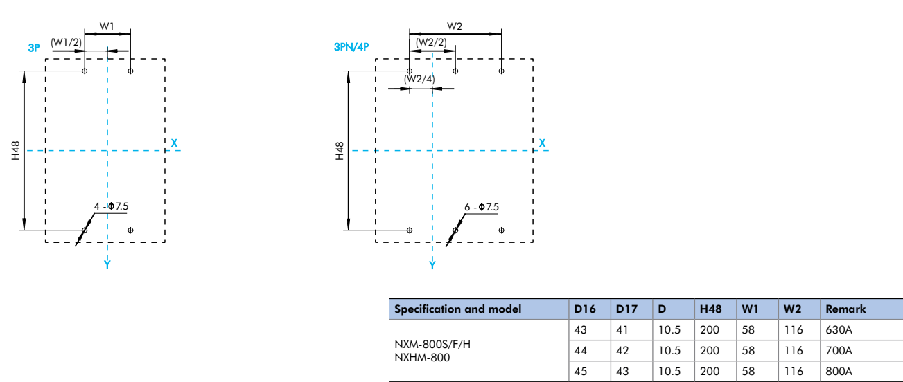
Installation size of baseplate(mm)
