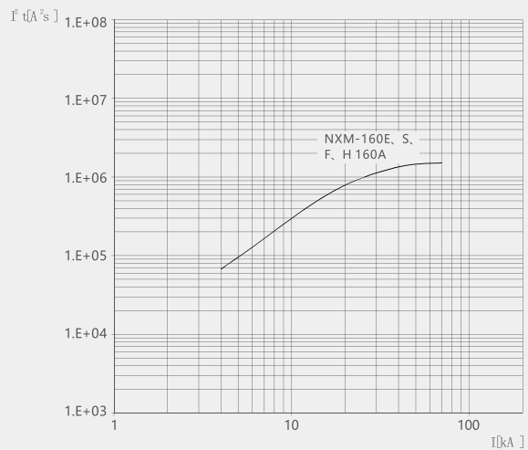
NXM-160 let-through energy curve
