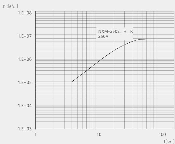
NXM-250 let-through energy curve
