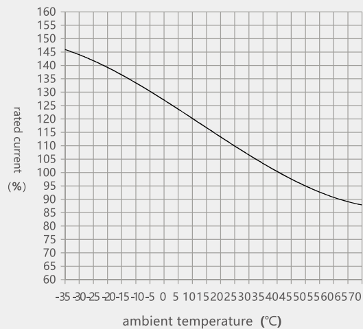
NXM-1000 Temperature compensation curve
