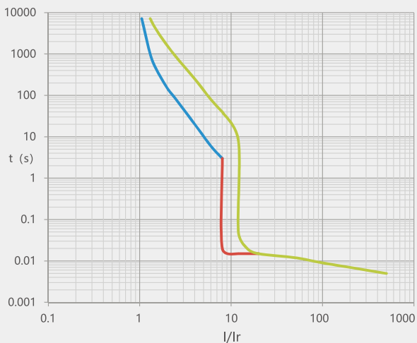
NXM-1250, 1600 Power distribution protection tripping curve
