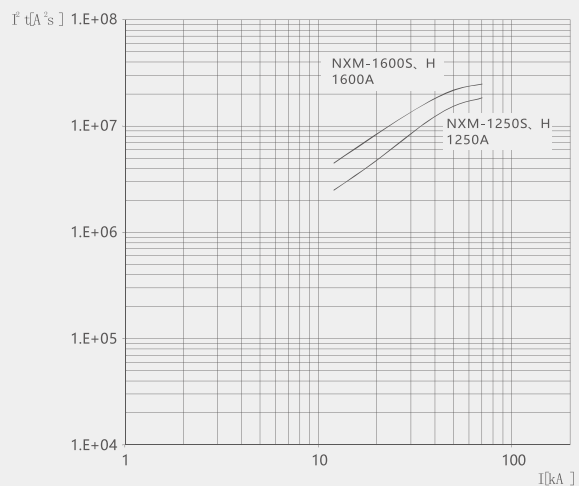
NXM-1250/1600 let-through energy curve
