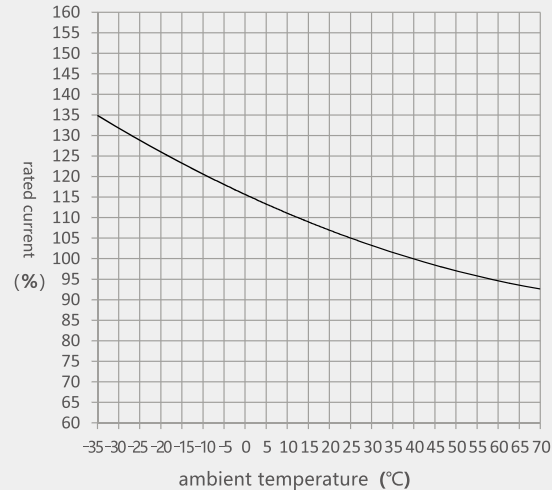
NXM-1250, 1600 Temperature compensation curve
