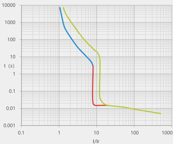
NXM-1000 Power distribution protection tripping curve
