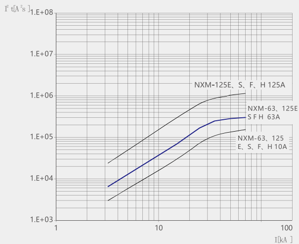
NXM-125 let-through energy curve
