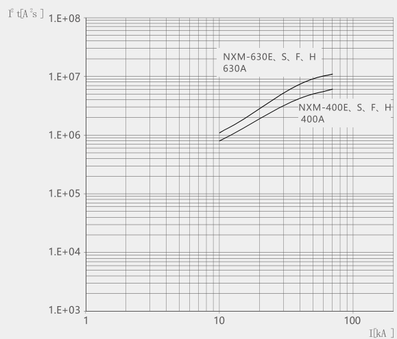
NXM-400/630 let-through energy curve
