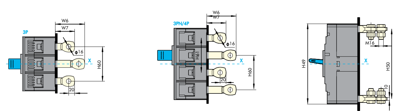
Rear connection, dimension (mm)
